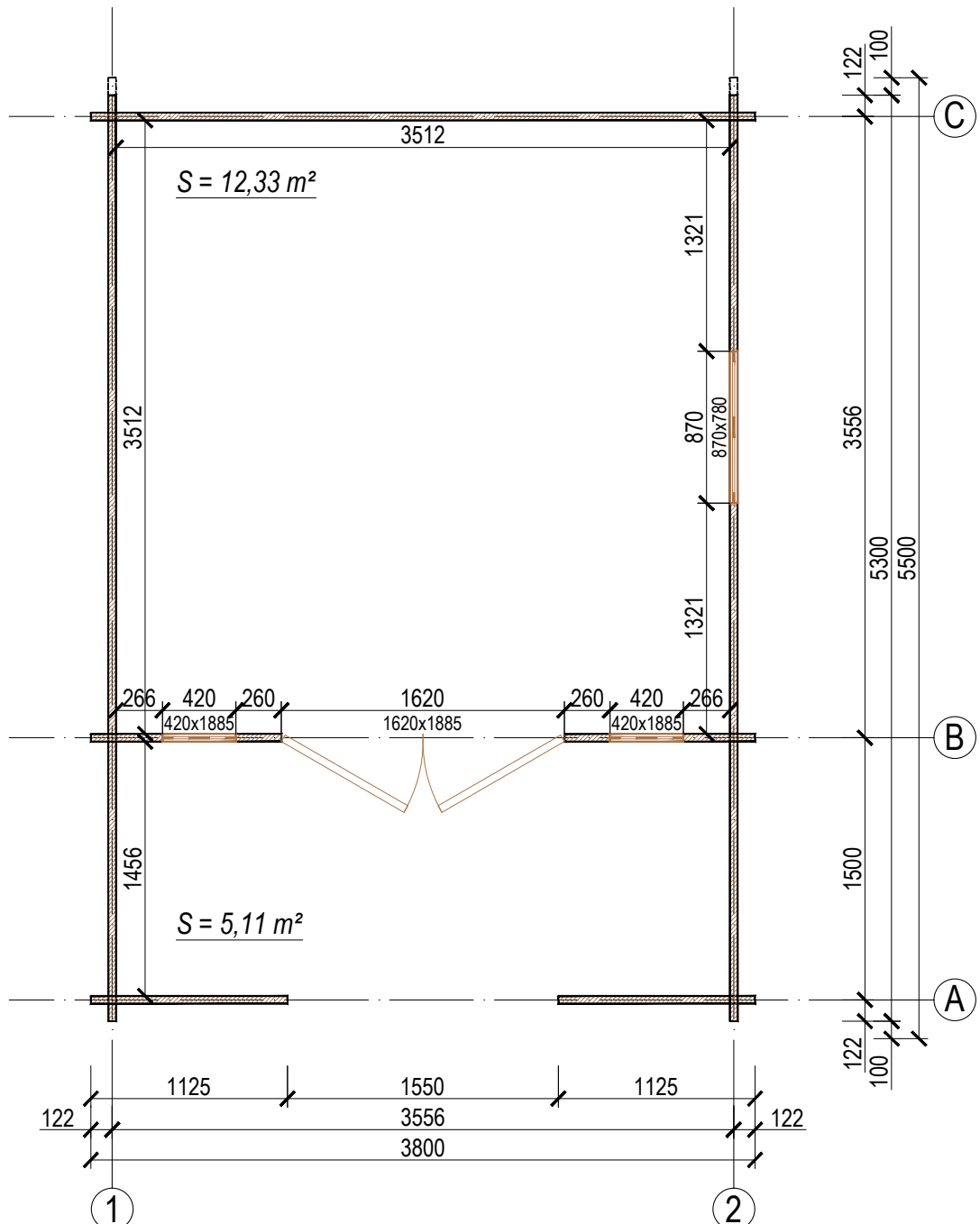
Plan of the axes 1/2 - A/C GH 016 - 3,8x3,8+1,5 - 44x130
