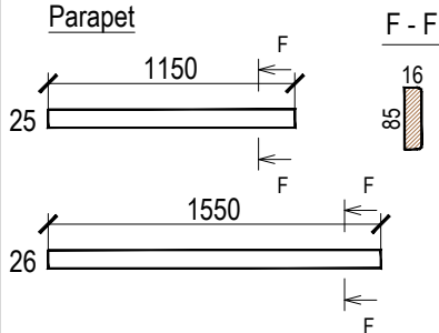
Plank
