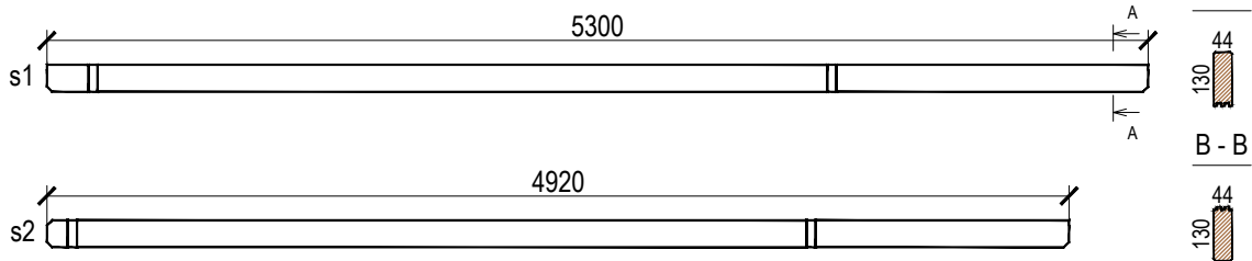
Rafter 44x135
